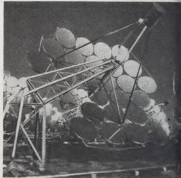
• The mylar film reflectors [above], which were the product of five years and $15 million of research and development, can be seen in this photo. According to LaJet , the low-cost concentrators reduced the per-watt installation cost of a solar power plant by some 80 percent.
